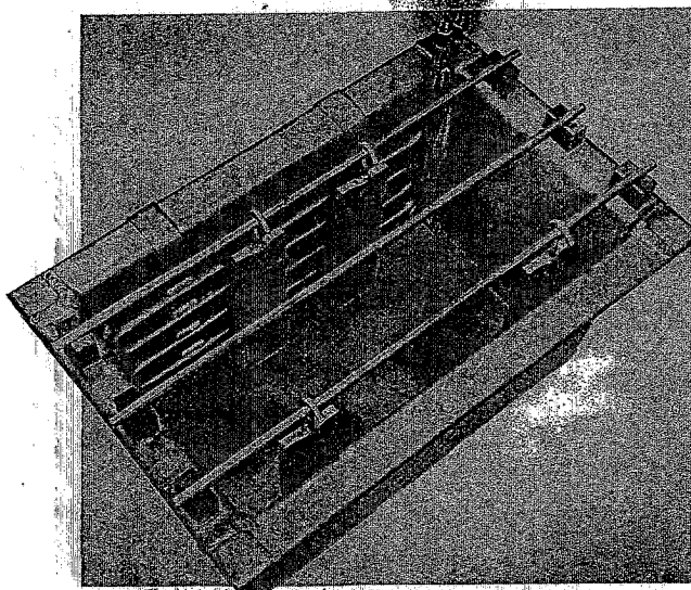
Small plating tank with Nalco Metal linings, coil and anodes . . . built to last.
