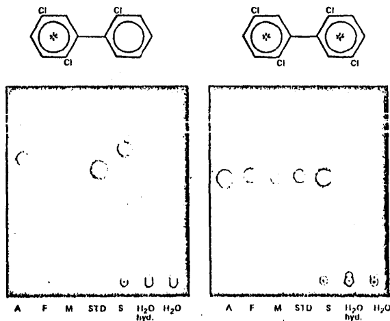
Fig. 2A. Radioautogram of TLC plate containing extracts of water and organisms treated with 2,5,2',5'-trichlorobiphenyl. A (alga), F (fish), M (mosquito larva), S (snail) and STD ( ^{14}\text{C} -radiolabeled compound).
