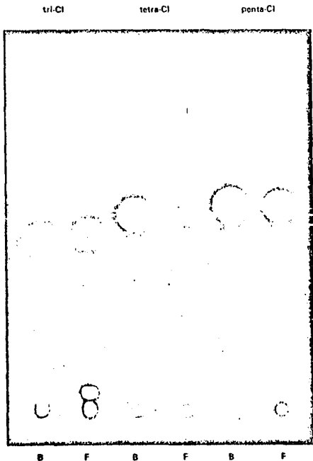
Fig. 3. Radioautogram of TLC plate containing extracts of bodies and feces of salt marsh caterpillar larvae fed ^{14} C-labeled 2,5,2'-tri-, 2,5,2',5'-tetra-, and 2,4,5,2',5'-pentachlorobiphenyls. B (body homogenate), and F (fecal excreta).
