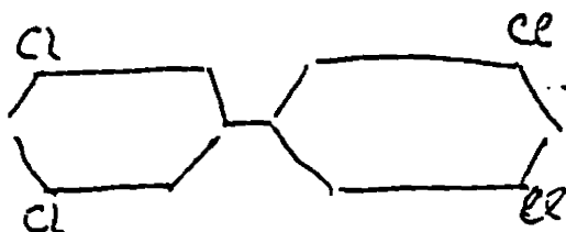
2, 2', 4, 4' - tetrachlorobiphenyl
