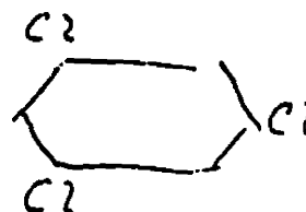
1, 3, 5 - trichlorobenzene
