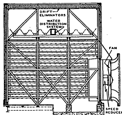
FIG. 7. FORCED DRAFT COOLING TOWER
