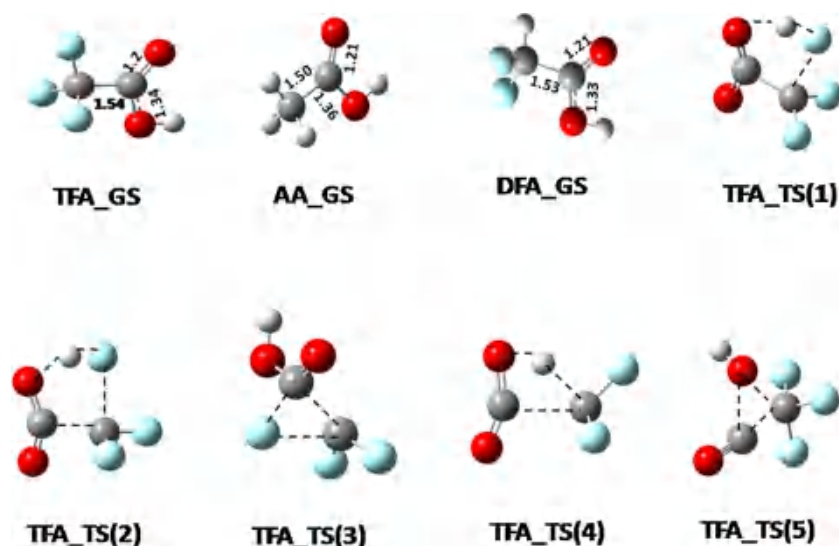
Fig. 7. Ground state structures of TFA, DFA and AA, (TFA_GS, AA_GS, DFA_GS,) optimized at the MP2/6-311+ + G** level of theory. The important transition states (TFA_TSs), for photodissociation of TFA at 193 nm are also geometry optimized at the MP2/6-311+ + G** level of theory. Details are given in the text.
