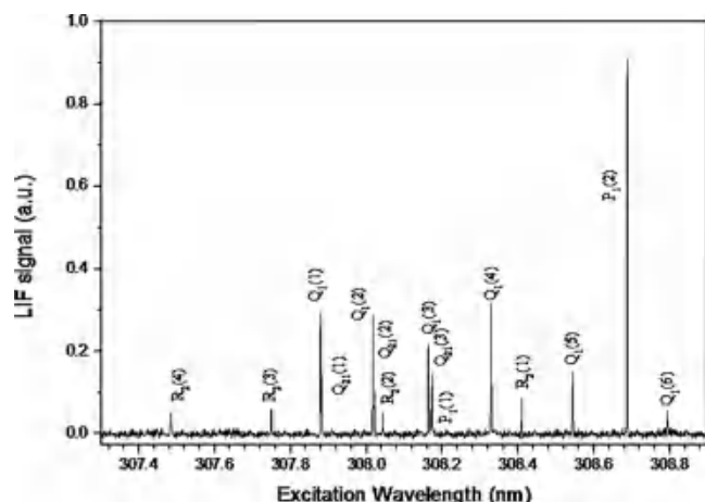
Fig. 1. A portion of the fluorescence excitation spectrum of the (0, 0) band of the A^2\Sigma^+ \leftarrow X^2\Pi (0,0) system of OH, generated in photodissociation of TFA at 193 nm. The pressure of TFA was maintained at around 10 mTorr, and pump-probe delay was kept at around 50 ns.
