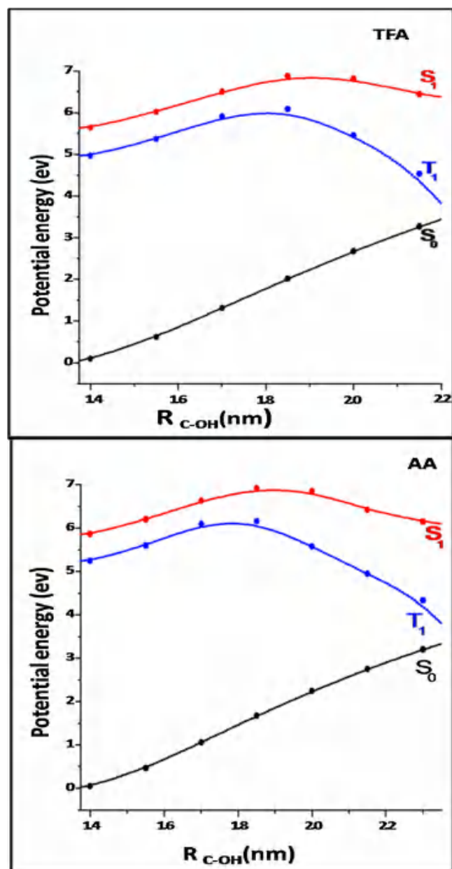
Fig. 9. Potential energy curves for the ground and the lowest singlet and triplet excited electronic states ( S_0 and T_1 ) of TFA and AA calculated with the time-dependent B3LYP/ aug-cc-pvdz method as a function of the CeOH bond length. The geometry was frozen to the equilibrium position of the respective states except for variation in the CeOH bond distance. The potential energy of the excited states are calculated by adding the vertical excitation energy to the energy of the respective ground state structure at each point.
