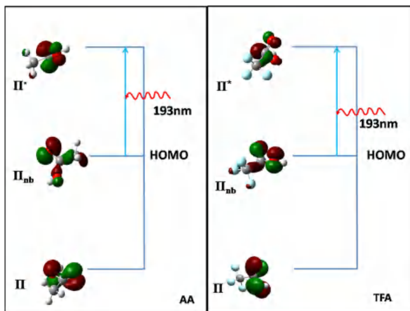
Fig. 8. The \pi(\text{HOMO}-1) , \pi_{\text{nb}}(\text{HOMO}) , and \pi^*(\text{LUMO}) orbitals of AA and TFA involved in the lower energy electronic transitions. The n\text{-}\pi^* transition to S_1 state populated by absorption at 193 nm is indicated in the figure.
