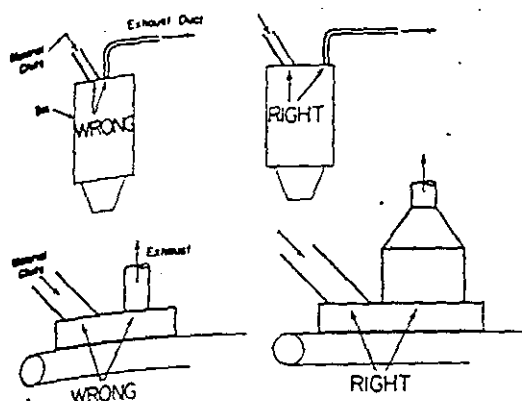
FIG. 2.—Needless product removal by exhaust system.
