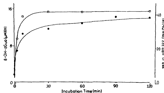
FIGURE 4: Time course of formation by singlet oxygen of 8-OH-dGuo and single-strand breaks. Deoxyguanosine (1 mM) or plasmid pBR322 DNA (2 \mu\text{g} ) was exposed to 40 mM \text{NDPO}_2 in 50 mM sodium phosphate buffer in \text{D}_2\text{O} (pH 7.4) at 37 ^\circ\text{C} .
