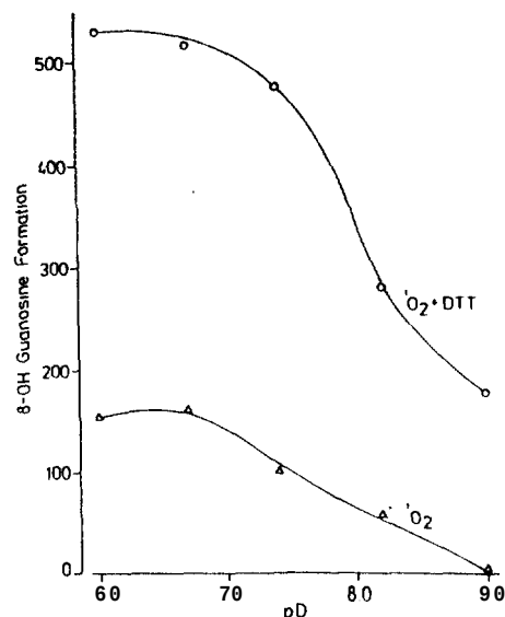
FIGURE 5: pH dependence of singlet oxygen induced (A) and singlet oxygen/thiol (O 2 ·DTT) induced 8-hydroxyguanine formation. Conditions are as in Figure 4; incubation was for 1 h at 37 ^\circ\text{C} . The value obtained with ^1\text{O}_2 at pH 7.4 (15.2 \mu\text{M} ) was taken as 100%. Dithiothreitol (DTT) concentration was 10 mM.
