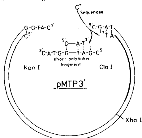
Scheme 1: Plasmid pMTP3' Used for Detection of Single-Strand Breaks by End Labeling
