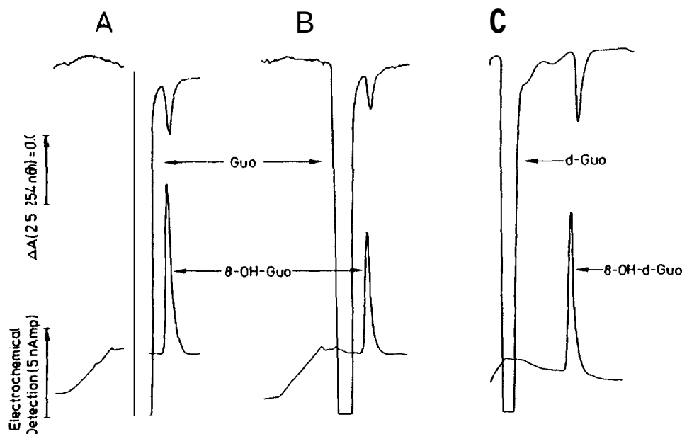
FIGURE 2: Detection by HPLC of the 8-OH-Guo (A, B) and 8-OH-dGuo (C) formation from Guo or dGuo. Singlet oxygen was generated from \text{NDPO}_2 (40 mM) in 50 mM sodium phosphate buffer, pH 7.4 in \text{D}_2\text{O} (A, C) or \text{H}_2\text{O} (B). Detection was by UV absorbance (top) and electrochemistry (bottom).
