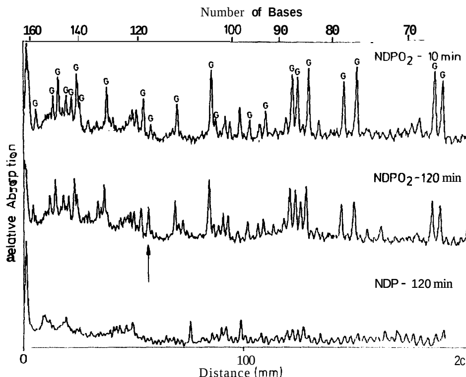
FIGURE 7: Laser densitometer scans of the autoradiograph of the gel with pMTP3' DNA treated with NDPO, for 10 and 120 min and NDP for 120 min. The G signal at position 117 differs significantly between the 10- and 120-min lanes (arrow).
