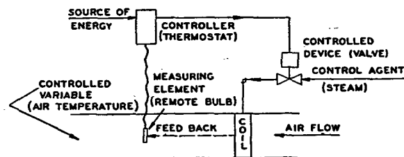
FIG. 1. ESSENTIALS OF A CONTROL SYSTEM
