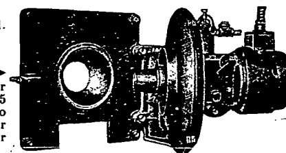
↑ TYPE 30 AV Fully automatic. Burns No. 5 Oil. Six sizes, 2 to 100 gph.
