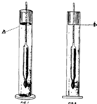
Method of Reading Baume Hydrometer
