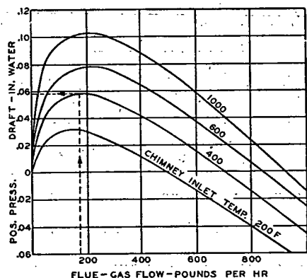
FIG. 4. AVAILABLE CHIMNEY DRAFT FOR 13 FT BRICK CHIMNEY a, b
