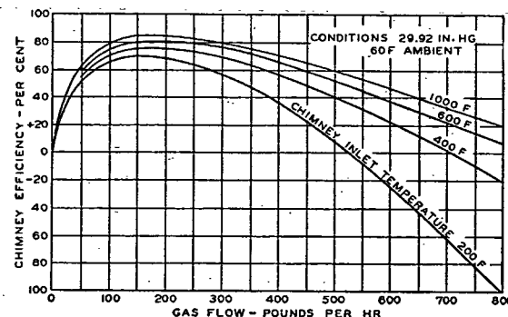
FIG. 5. EFFECT OF GAS FLOW ON CHIMNEY EFFICIENCY a
