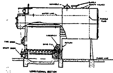
"5000" Series Diagram Welded Firebox Boilers Updraft 5178-5190 Mechanical ratings same dimension as 5078-5090 Hand-fired. Smokeless Downdraft 5177-5190 Mechanical rating same dimensions as 5077-5090 Hand-fired.
