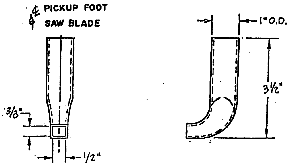
PICKUP FOOT-WELDED TO SHIELDING
