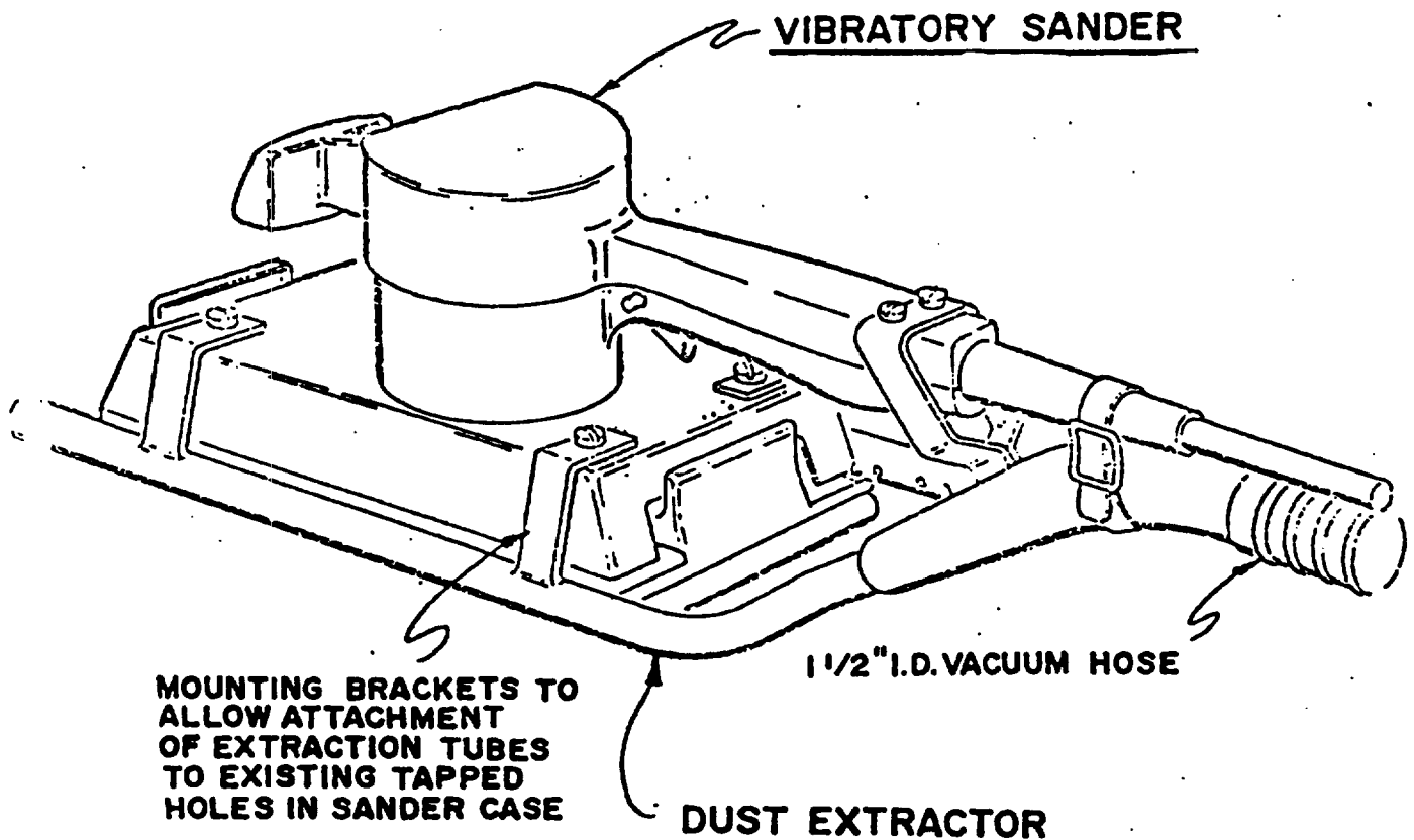
DUST EXTRACTOR — VIBRATORY SANDER
