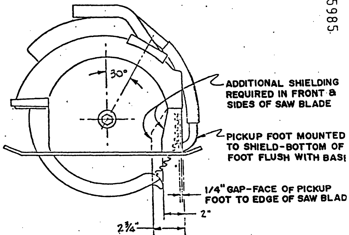
DUST EXTRACTOR-PORTABLE SAW-7 1/4" DIA. BLADE
