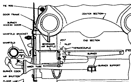
FIG. 7—Burner No. 2 and Pilot Installation—Manual Ignition
