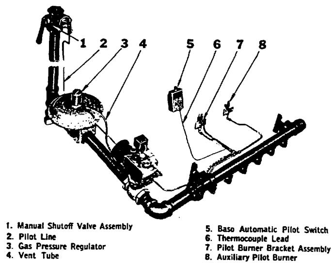
FIG. 16—Control Connections
