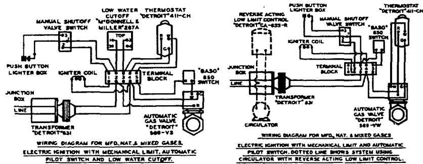
FIG. 13—Wiring Diagrams (Electric Ignition)
