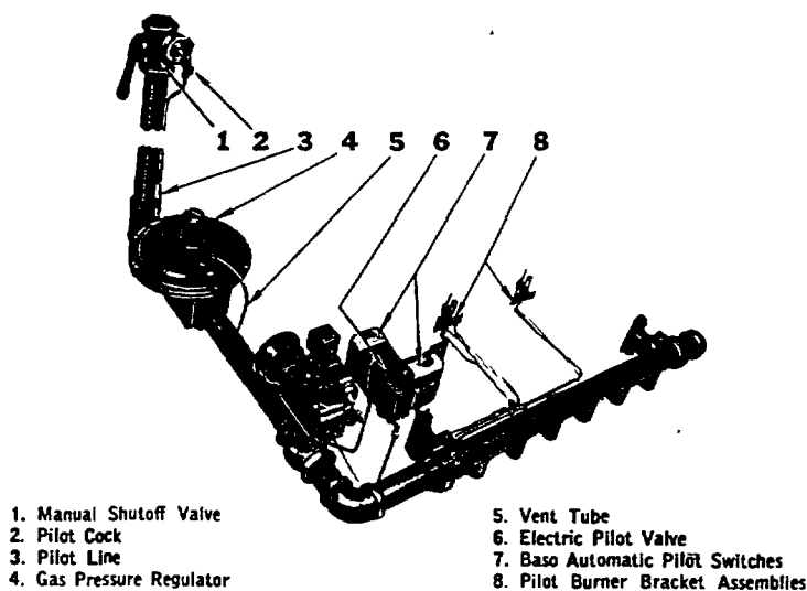
FIG. 21—Control Connections
