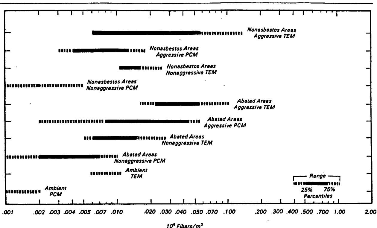
Figure 1. Comparison of airborne fiber concentrations for PCM and TEM under static (nonaggressive) and aggressive conditions.
