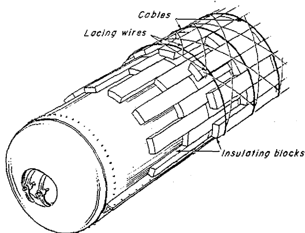
CYLINDRICAL SURFACE of steam drum using double-layer insulation. Blocks are held by wire laced to anchored cable
