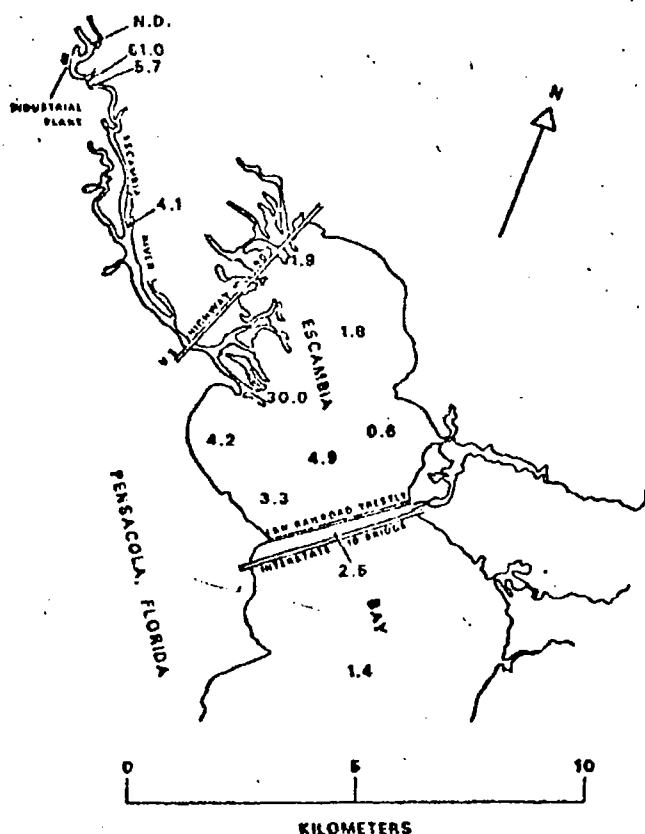
Fig. 1 Study area showing lower Escambia River, upper Escambia Bay and stations where sediment was collected on February 24, 1970. The amount of 'Aroclor 1254' found at each station is given in parts per million (p.p.m.). ND, Not detected.
