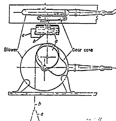
Figure 1.—Apparatus for measuring the flow required to operate blower. (COPD, Part 11, Subpart J, § 11.124-2)
