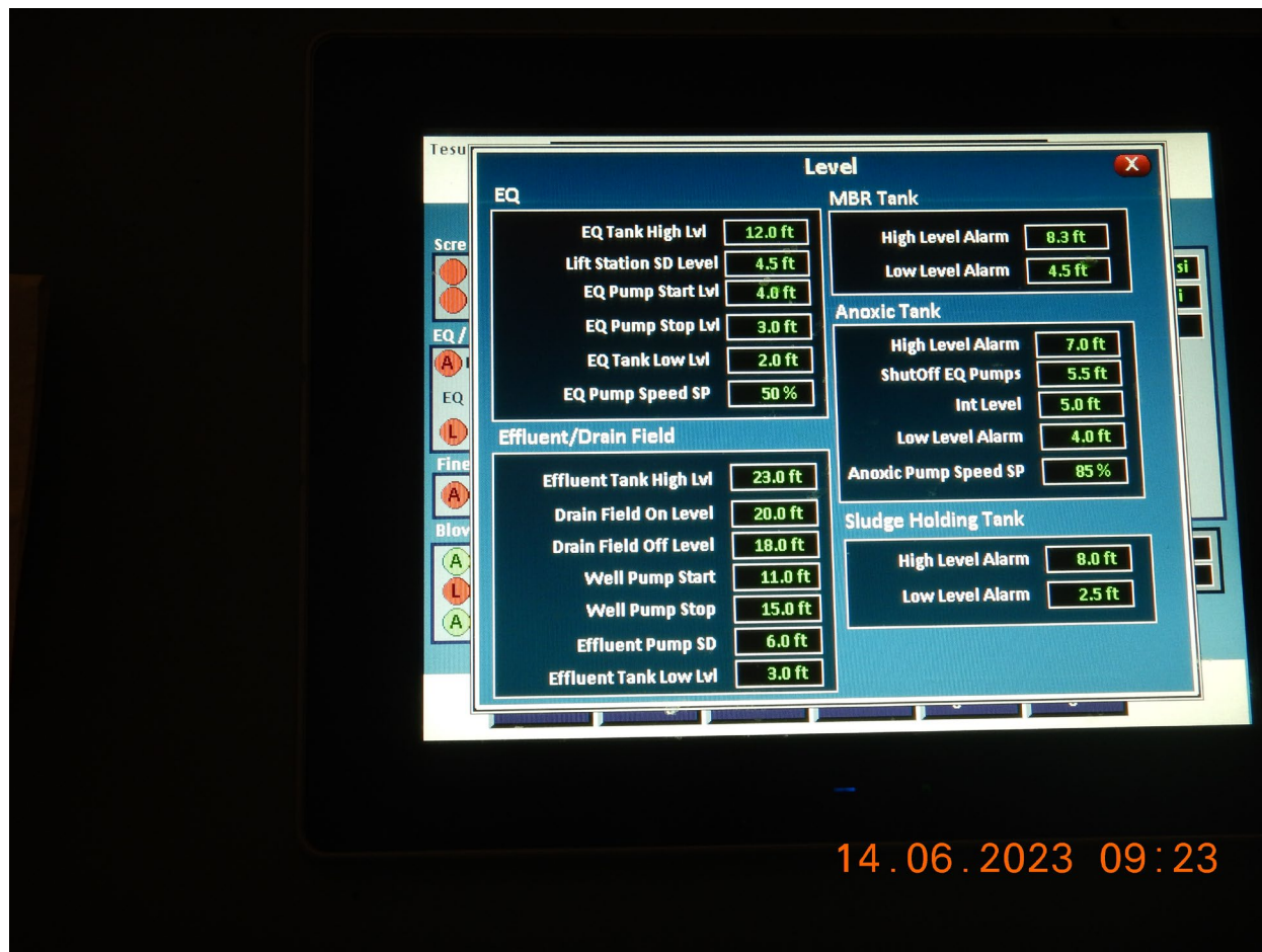
View of the Supervisory Control and Data Acquisition (SCADA) system. (DSCN2574) Photographed by D. Esparza
