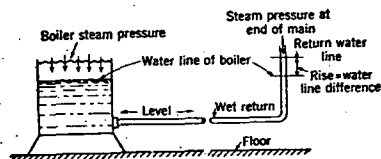
FIG. 1. DIFFERENCE IN STEAM PRESSURE ON WATER IN BOILER AND AT END OF STEAM MAIN
