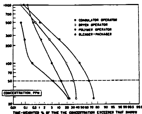
FIGURE 2. Exposure profiles expressed as VCI vapor concentration versus the exposure frequency distribution for the four job classifications.
