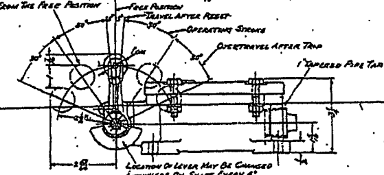
Snap Action Limit Switch with roller lever operator.
