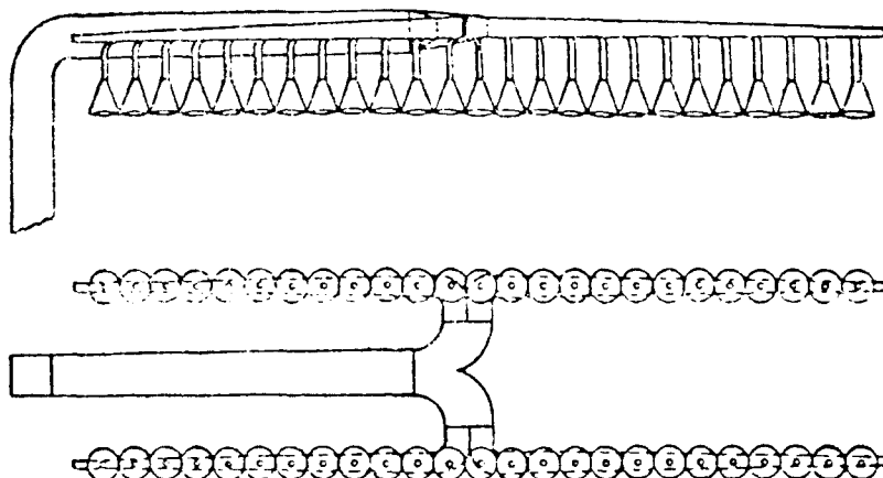
FIGURE 8—Schematic views of exhaust system applied to Foster winders.
