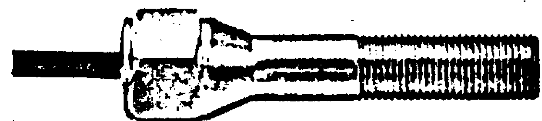
Model 713560 \frac{1}{2} NPT conduit outlet with 18" 3 conductor cable, type 300 stainless steel housing with \frac{1}{2} -18 NF x 1.5" threads with 2 lock nuts.
