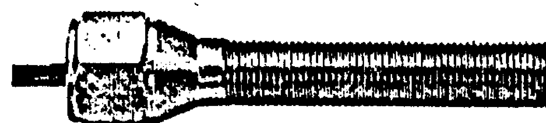
Model 713770 \frac{1}{2} NPT conduit outlet, 18" potted 3 wire leads, type 300 stainless steel housing with \frac{1}{2} -18 NF x 2.813" threads with 2 lock nuts.
