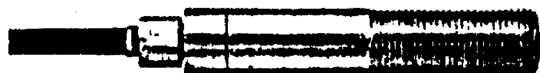
Model 713360 No conduit connection, 18" 3 conductor cable with water resistant squeeze connection, type 300 stainless steel housing with \frac{1}{2} -18 NF x 1.5" threads with 2 lock nuts.
