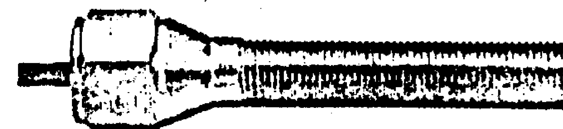
Model 713774 \frac{1}{2} NPT conduit outlet with 18" potted, 3 wire leads, type 300 stainless steel housing with \frac{1}{2} -18 NF x 2.813" threads.
