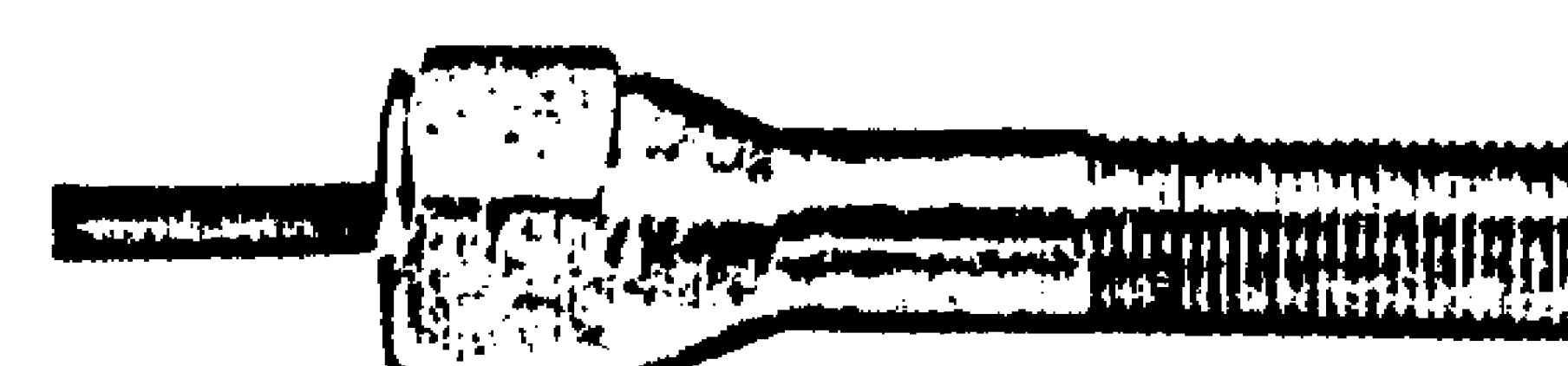
Model 713764 \frac{1}{2} NPT conduit outlet with 18" potted, 3 wire leads, type 300 stainless steel housing with \frac{1}{2} -18 NF x 1.5" threads with 2 lock nuts.
