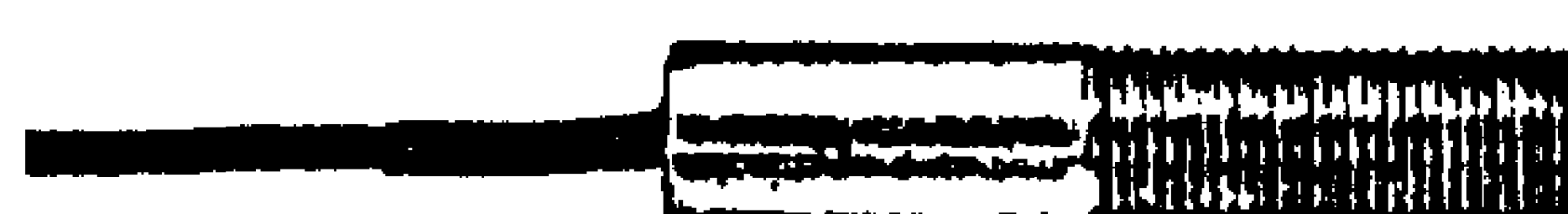
Model 713660 No conduit outlet, 18" potted, 3 wire leads, type 300 stainless steel housing with \frac{1}{2} -18 NF x 1.5" threads with 2 lock nuts.
