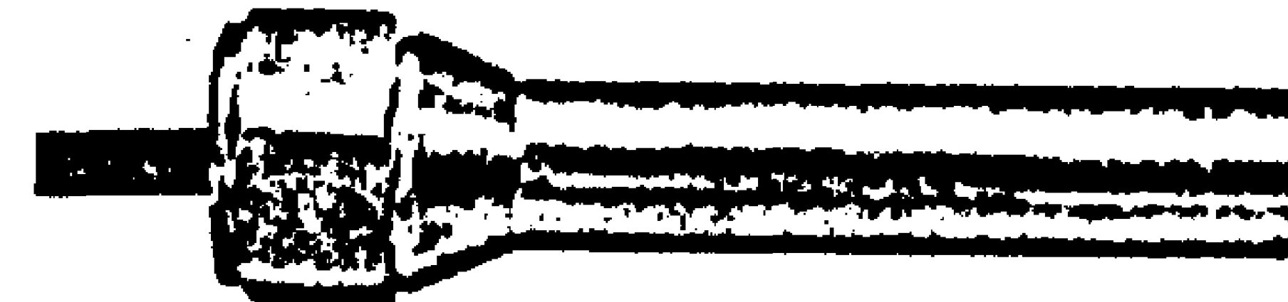
Model 713524 \frac{1}{2} NPT conduit outlet with 18" potted, 3 conductor cable, type 300 stainless steel housing, no threads.
