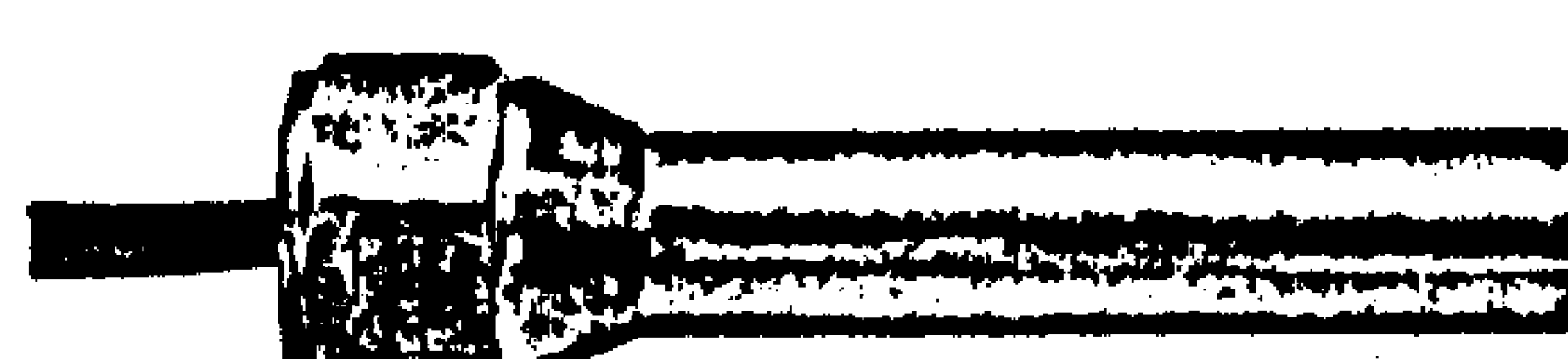
Model 713720 \frac{1}{2} NPT conduit outlet with 18" potted, 3 wire leads, type 300 stainless steel housing, no threads.
