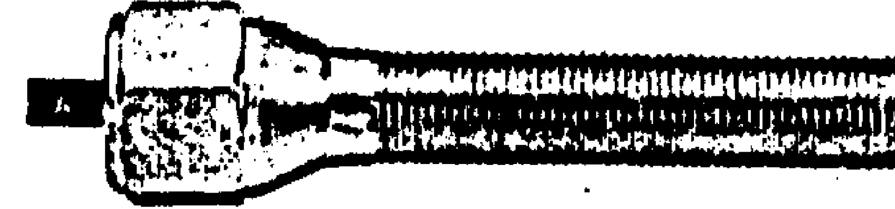
Model 713574 \frac{1}{2} NPT conduit outlet with 18" potted, 3 conductor cable, type 300 stainless steel housing with \frac{1}{2} -18 NF x 2.813" threads with 2 lock nuts.
