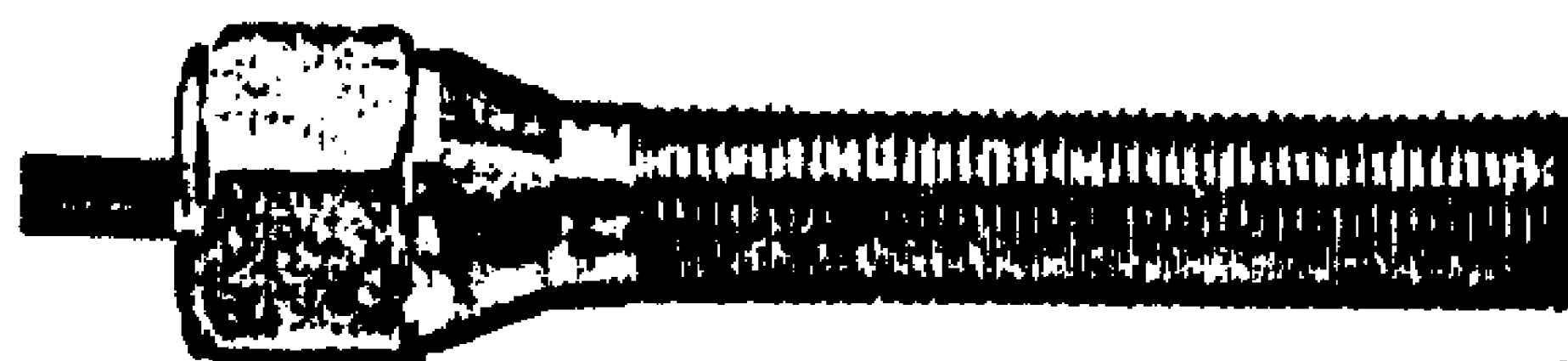
Model 713570 \frac{1}{2} NPT conduit outlet, 18" 3 conductor cable, type 300 stainless steel housing with \frac{1}{2} -18 NF x 2.813" threads with 2 lock nuts.
