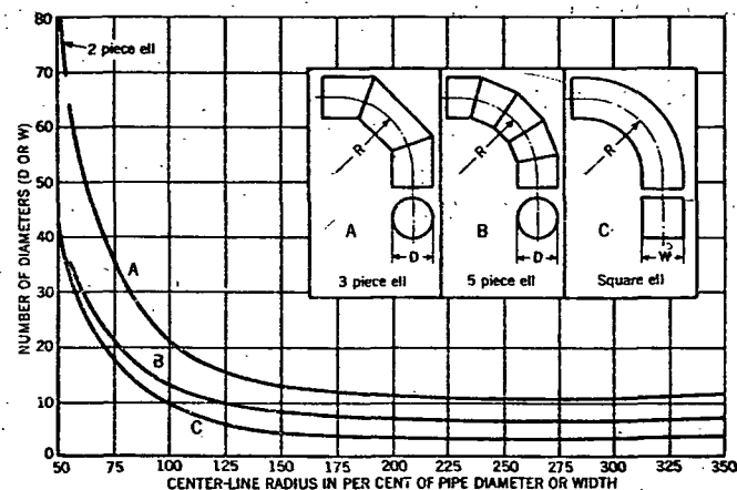
FIG. 6. LOSS OF PRESSURE IN ELBOWS
