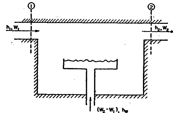
FIG. 2. ILLUSTRATION OF ADIABATIC SATURATION
