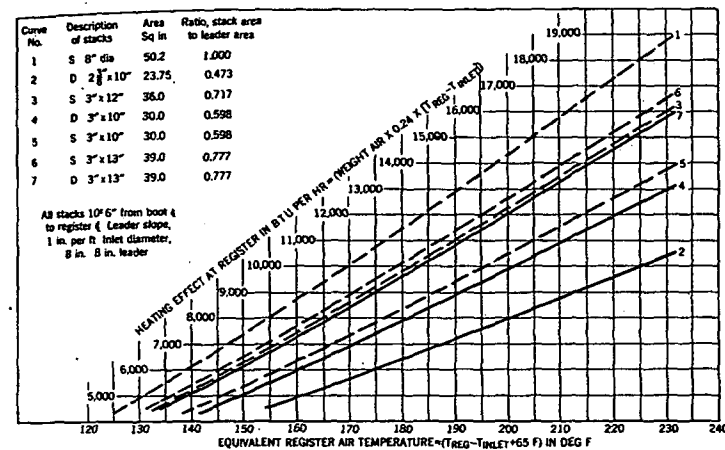
FIG. 5. HEATING EFFECT AT REGISTERS FOR VARIOUS STACKS WITH 8-IN. LEADER
