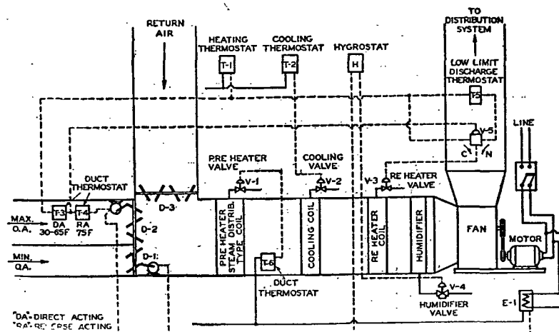
FIG. 1. CONTROL DIAGRAM FOR YEAR 'ROUND AIR CONDITIONING SYSTEM
