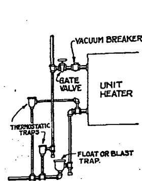
FIG. 1. UNIT HEATER CONNECTIONS WHERE CONDENSATION IS RETURNED TO VACUUM PUMP
