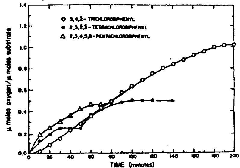
Figure 2. Oxidation of tri, tetra, and penta chlorobiphenyl.
