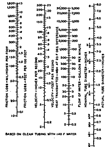
Fig. 4....Friction Loss Due to Flow of Water in Type L Copper Tube 1
