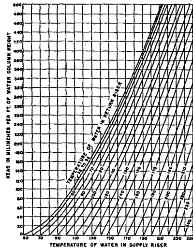
Fig. 1....Heads Resulting from Temperature Difference (Gravity Systems)
