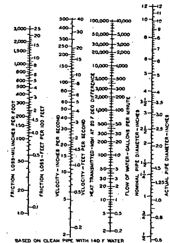
Fig. 3....Friction Loss Due to Flow of Water in Iron Pipe 1,3
