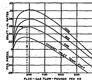
Fig. 6.... Available Chimney Draft for 13 Ft Brick Chimney.*
