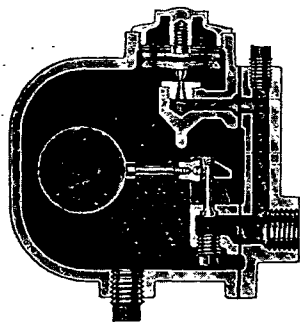
Fig. 6. Webster Size 00026-T Drip Trap has rated capacity of 200 lb Water per Hour at 2 lb Pressure Difference
