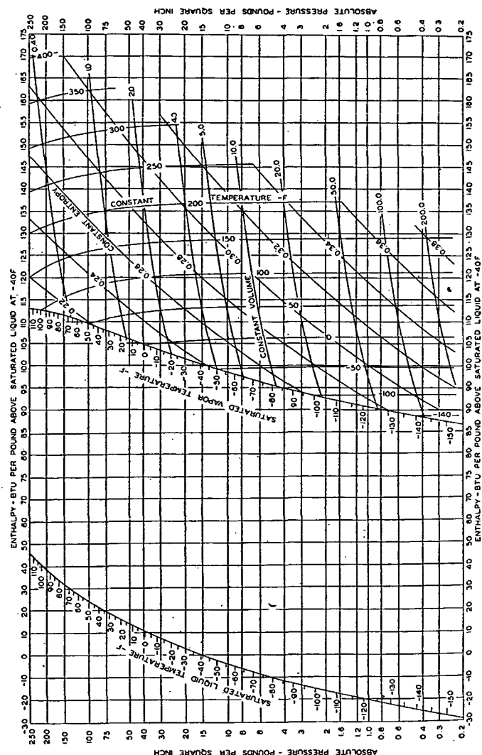
Fig. 2. Pressure-Enthalpy Diagram for Monochlorodifluoromethane (CHClF 2 ) (Refrigerant 22) Temperature—F; Volume—Cu Ft per Lb, Entropy—Btu per (Lb)(F deg).
