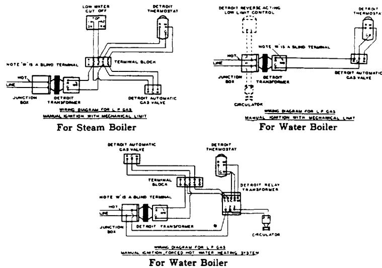
FIG. 19—Wiring Diagrams (Manual Ignition)
