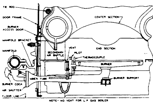
FIG. 7—Burner No. 2 and Pilot Installation-Manual Ignition
