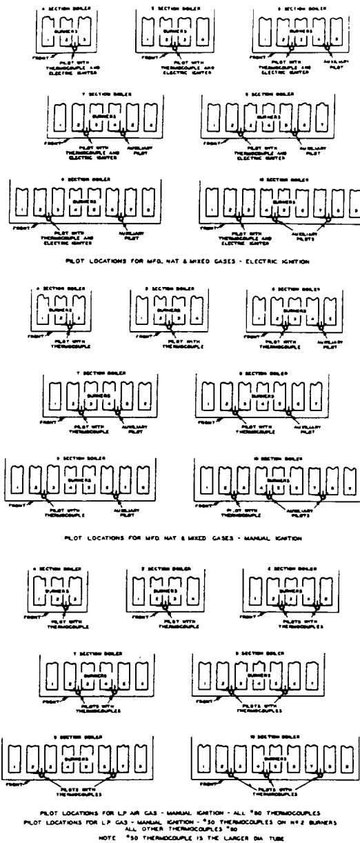
FIG. 5—Burner and Pilot Locations
