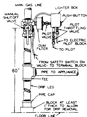
FIG. 14—Supply Piping Electric Ignition
