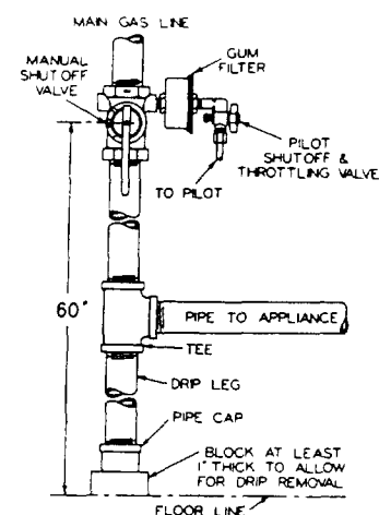
FIG. 15—Supply Piping Manual Ignition
