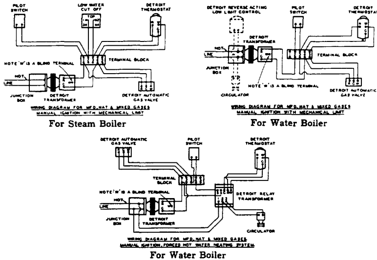
FIG. 17—Wiring Diagrams (Manual Ignition)
