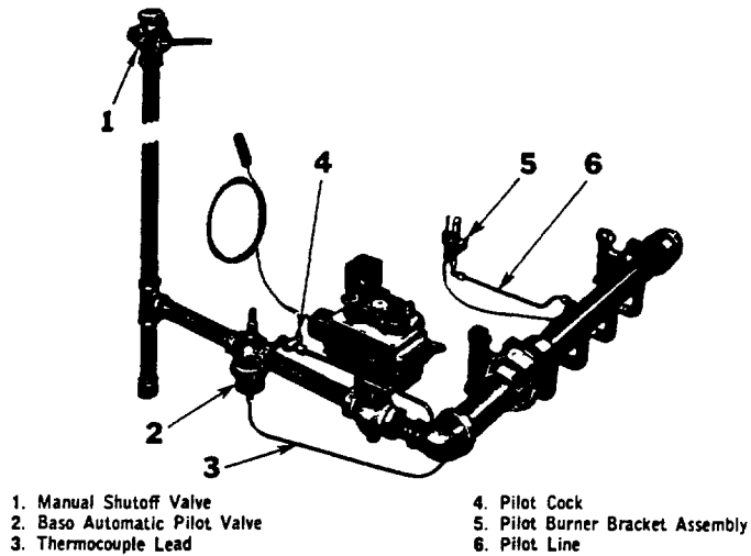
FIG. 18—Control Connections
