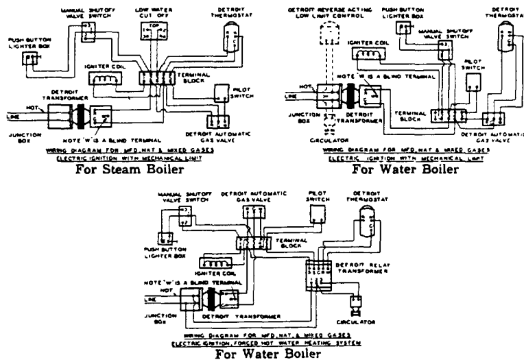
FIG. 13—Wiring Diagrams (Electric Ignition)
