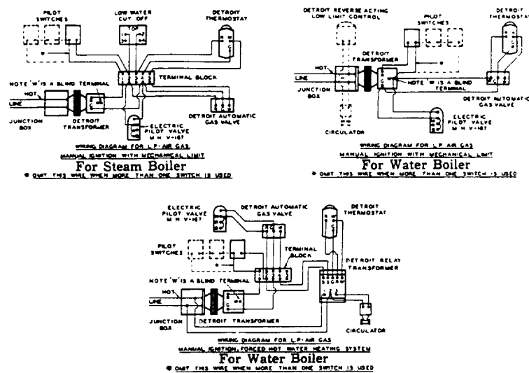
FIG. 22—Wiring Diagram (Manual Ignition)
