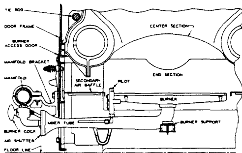
FIG. 8—Burner and Auxiliary Pilot
