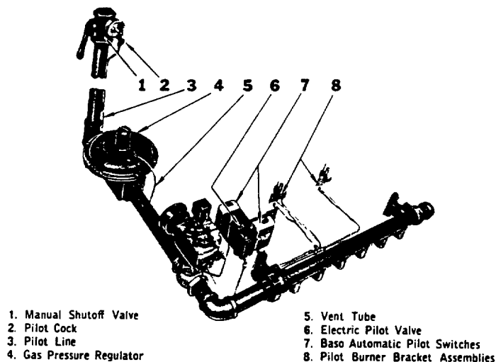
FIG. 21—Control Connections
