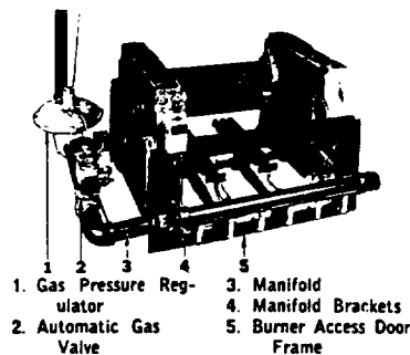
FIG. 4—Manifold and Piping
