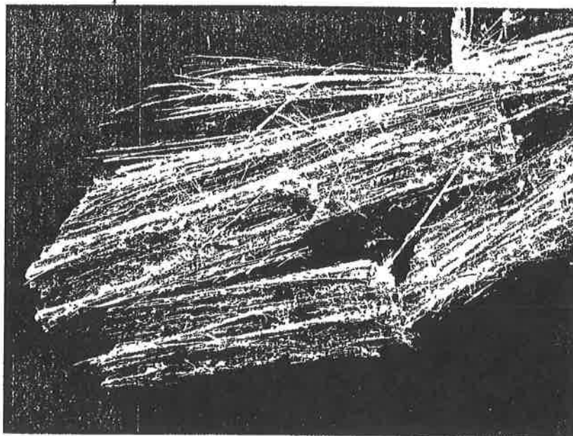
FIGURE 4; - Macrophotographs (X 3) of anthophyllite (top) and anthophyllite asbestos (bottom);
