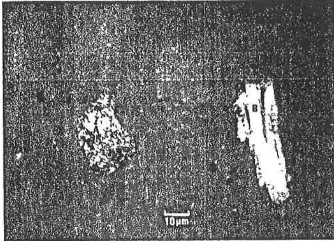
FIGURE 52. - Platy talc (A) and tremolite cleavage fragment (B) (X 640).
