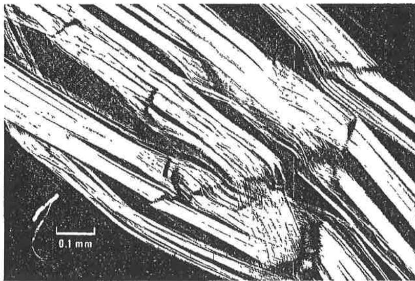
FIGURE 18. - Chrysotile by polarized light (X 100).
