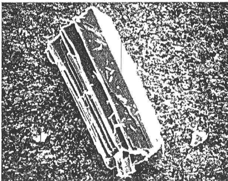
FIGURE 31. - Tremolite, showing good prismatic cleavage (SEM photomicrograph at X 560).
