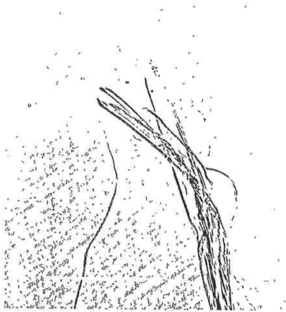
FIGURE 19. - Chrysotile (X 300).
