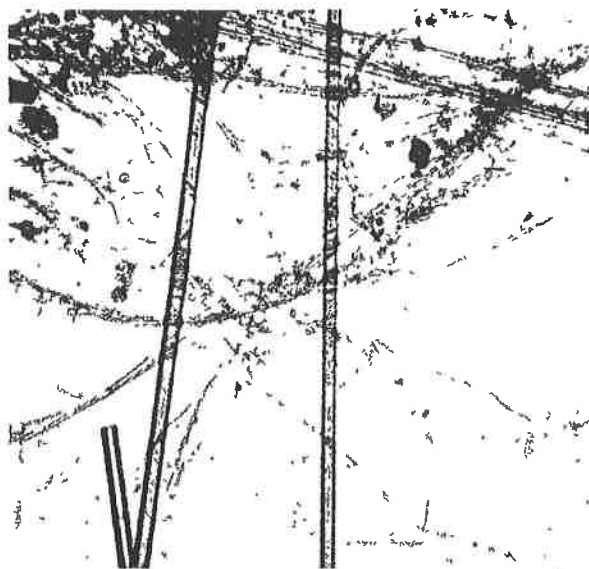
FIGURE 50. - Sample from university building, showing a mixture of chrysotile and fiberglass (X 140).
