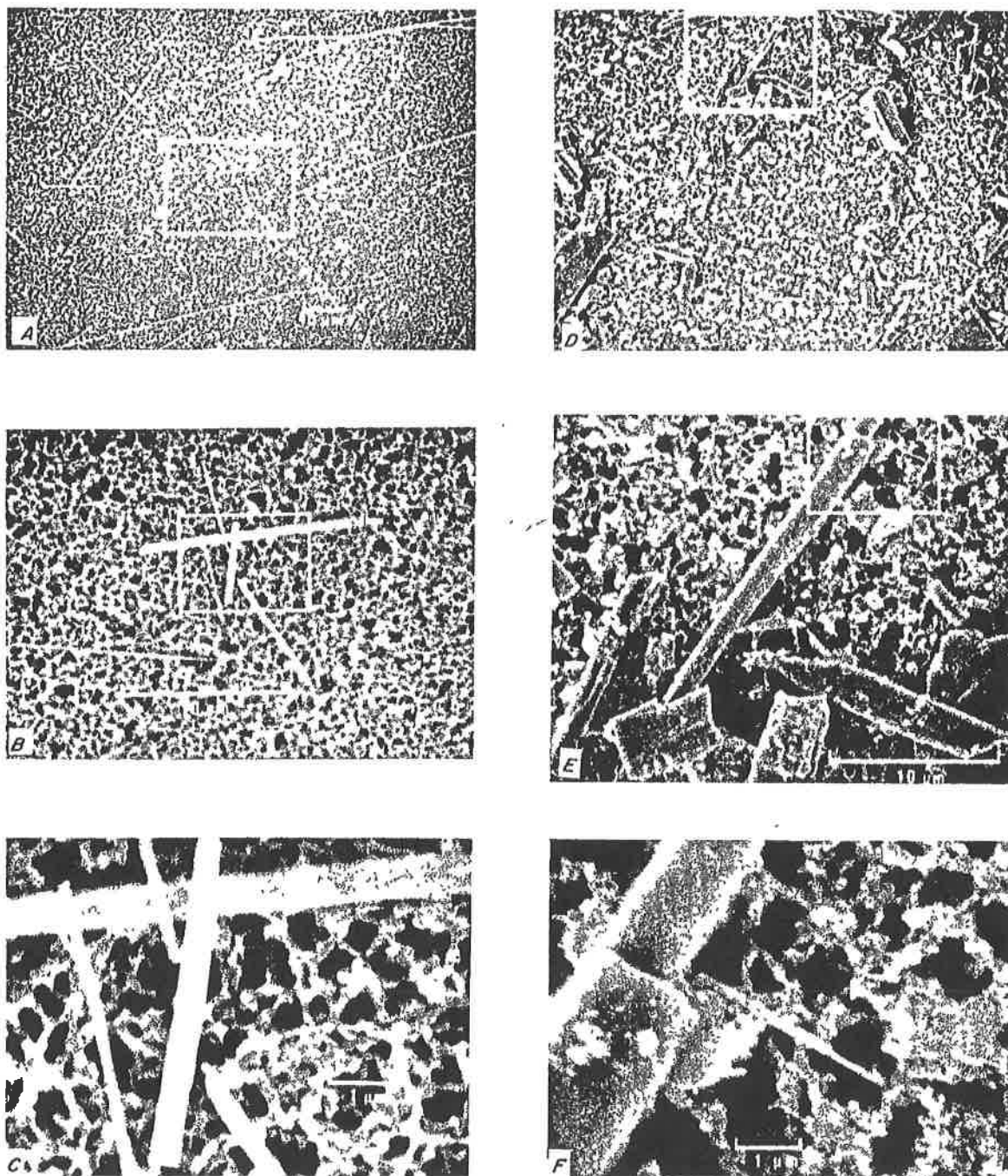
FIGURE 40. - SEM photomicrographs of crocidolite and riebeckite at three magnifications: Crocidolite (left) at A , X 500; B , X 2,500; and C , X 10,000. Riebeckite (right) at D , X 500; E , X 2,500; and F , X 10,000. Rectangles indicate the area shown at the next higher magnification.
