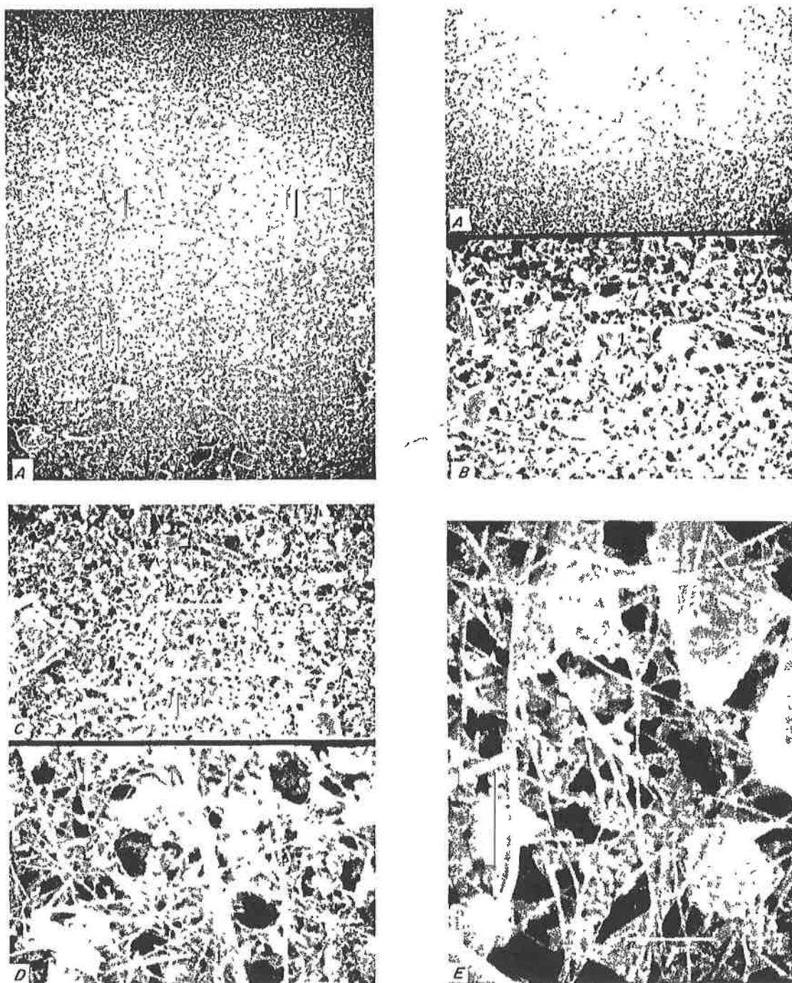
FIGURE 47. - Mixture of nonasbestiform serpentine and chrysotile at five magnifications: A, X 450; B, 2,250; C, X 9,000; D, 1,800; and E, X 18,000. Rectangles indicate the area shown in the next panel.
