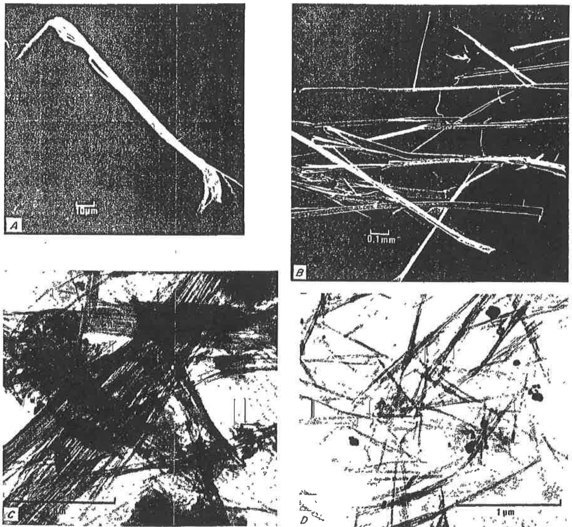
FIGURE 13. - Four fibrous nonasbestiform mineral varieties: A , Fibrous talc (X 500); B , fibrous brucite (X 50); C , palygorskite (X 30,000); and D , attapulgite (X 30,000).
