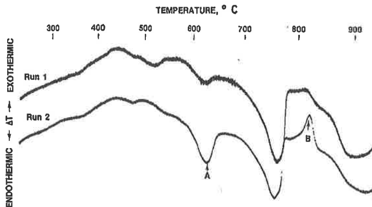
FIGURE 48. - Differential thermal analysis of sample from school ceiling, showing endothermic (A) and exothermic (B) peaks of serpentine. Run 1 is the sample as received; run 2 is a mixture of 95 pct of the as-received sample and 5 pct chrysotile.
