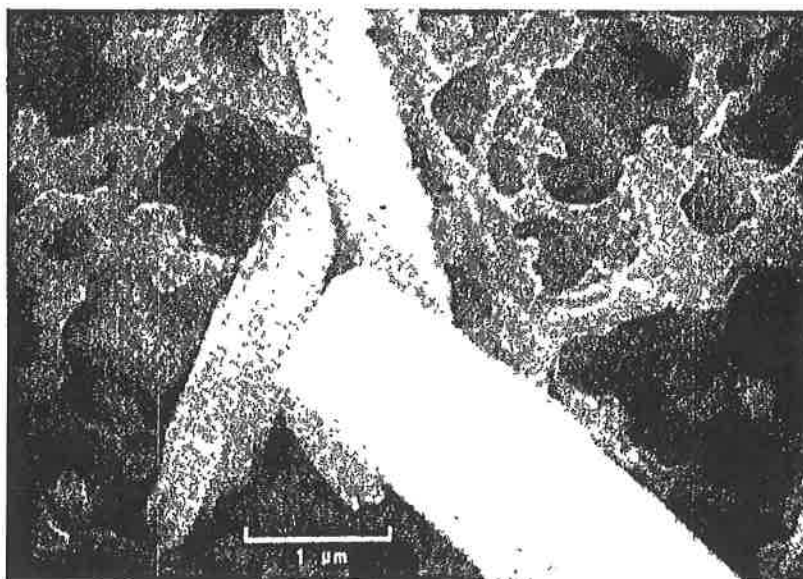
FIGURE 25. - Actinolite, showing prismatic shape (SEM photomicrograph at X 20,000).
