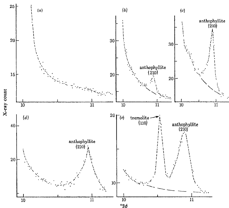
FIGURE 8. X-ray diffraction step scans of talc samples. ( a, b, c ) Representative dilution standards containing 1 %, 5 % and 10 % anthophyllite in talc. ( d, e ) Consumer talc powders purchased in New York City.
