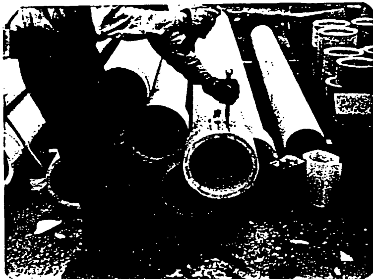
FIGURE 25. Removal of coupling with chisel.
