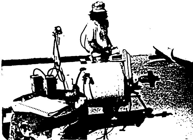
FIGURE 17. Use of manual lathe on 16-inch pressure pipe.
