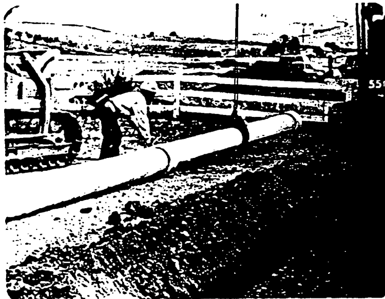
FIGURE 3. Placing pipe at side of trench.
