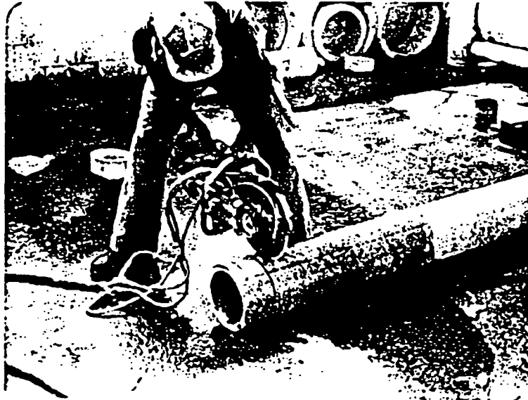
FIGURE 11. Use of abrasive disc saw, wet.
