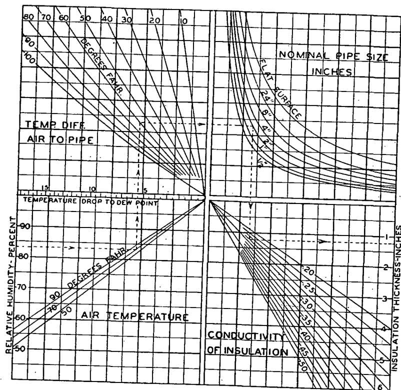
FIG. 4. THICKNESS OF PIPE INSULATION TO PREVENT SWEATING a
