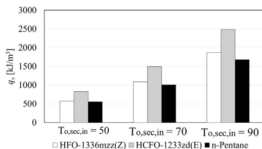
Fig. 8. Two-stage cycle with IHX simulations results of volumetric heating capacity for heating production.
