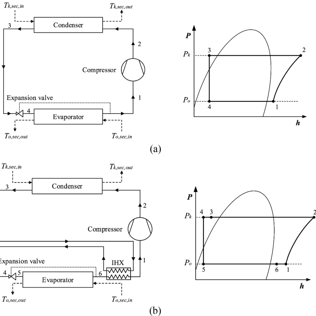
Fig. 1. Schematic and P-h diagram of single-stage configurations: (a) single-stage cycle and (b) single-stage cycle with IHX.
