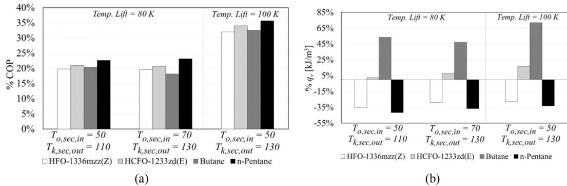
Fig. 6. Simulation relative results of COP and volumetric heating capacity for temperature lifts of 80 and 100 K.
