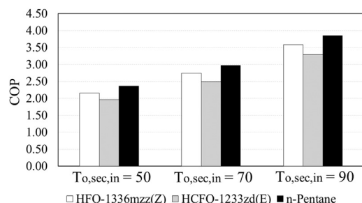
Fig. 7. Two-stage cycle with IHX simulations results of COP for heating production temperature of 150 °C.
