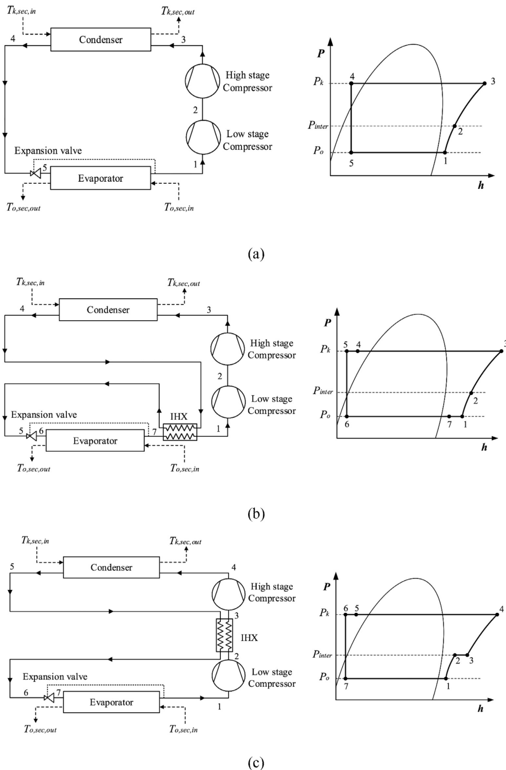
Fig. 2. Schematic and P-h diagram of two-stages configurations: (a) two-stage cycle, (b) two-stage cycle with IHX and (c) two-stage cycle with intermediate-IHX.
