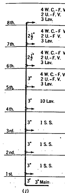
FIG. 5. UP-FEED SYSTEM
