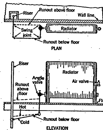
FIG. 44. ONE-PIPE RADIATOR CONNECTIONS
