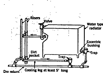
FIG. 45. TWO-PIPE TOP AND BOTTOM OPPOSITE END RADIATOR CONNECTIONS
