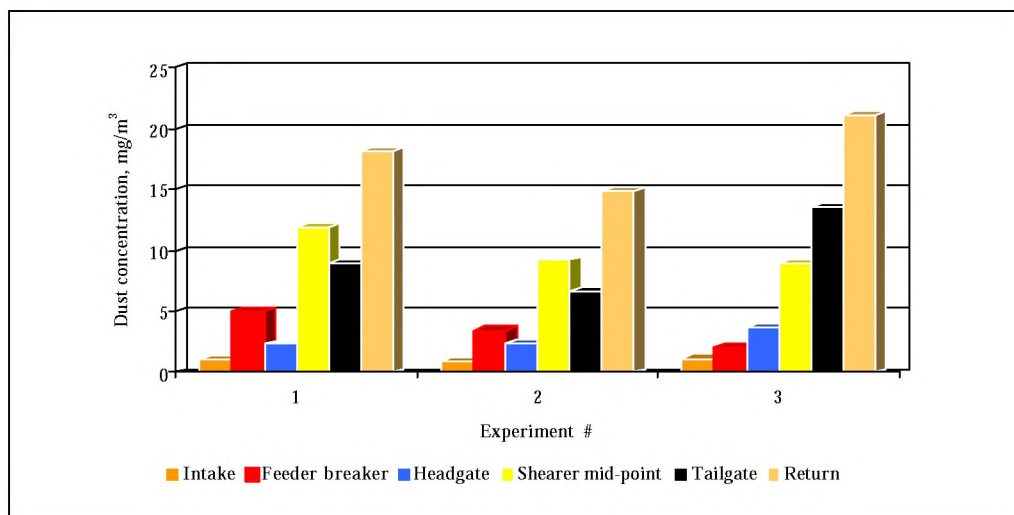
Figure 5.3b: Measured ARD concentrations (8-h) along the shortwall section
