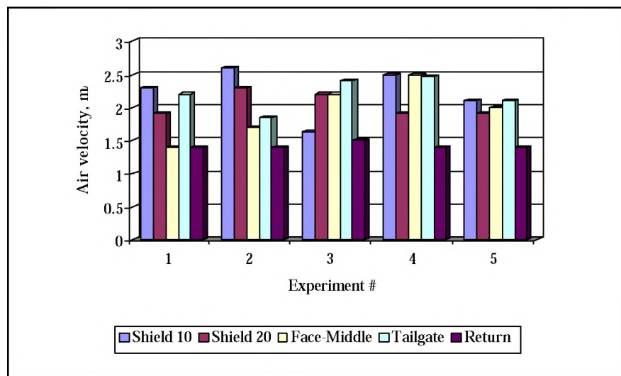
Figure 5.2.2a Measured air velocities along the shortwall section
