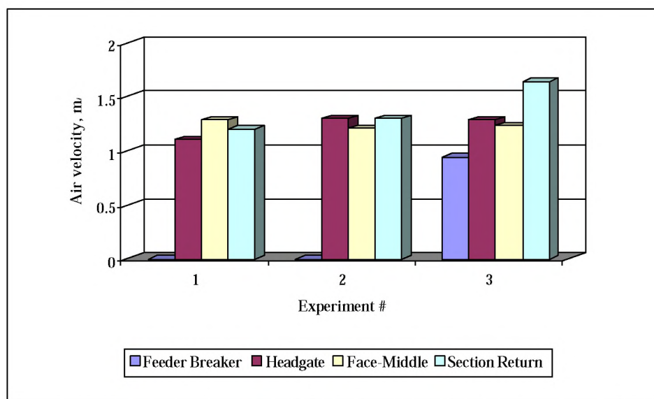
Figure 5.3a: Measured air velocities along the shortwall section
