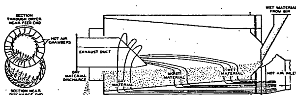
FIG. 12. CROSS SECTION AND LONGITUDINAL SECTION THROUGH CIRCULATION DRYER 8
