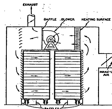
FIG. 13. COMPARTMENT DRYER, SHOWING TRUCKS, WITH AIR CIRCULATION 8
