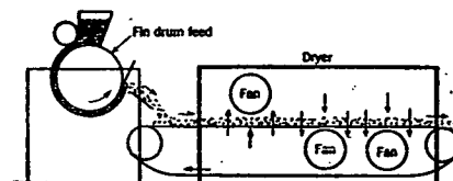
FIG. 14. SECTION OF CONTINUOUS DRYER, BLOW-THROUGH TYPE
