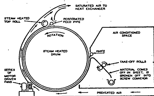
FIG. 11. DRUM DRYER 8
