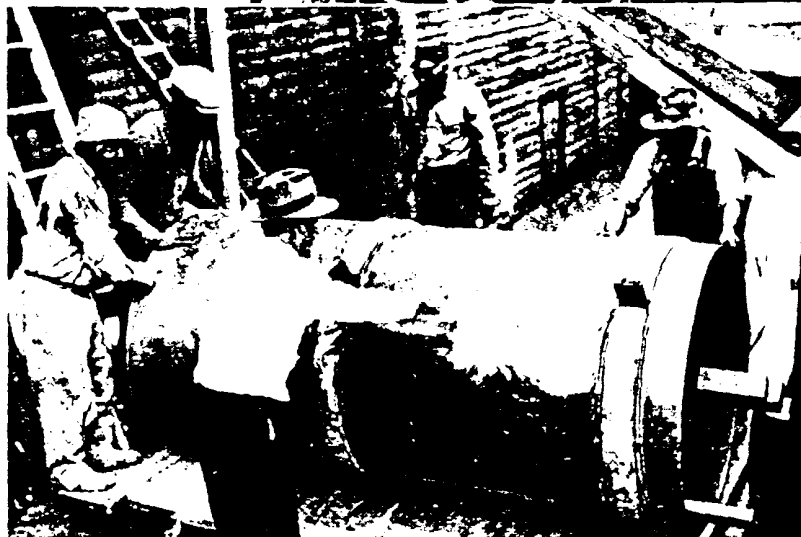
Below, preparing to remove the mandrel from a completed section of the lead duct. Note that steel straps which provide both stiffening and support are secured to the duct and sealed off from corrosive atmosphere by sheet lead covering burned to the duct wall.
