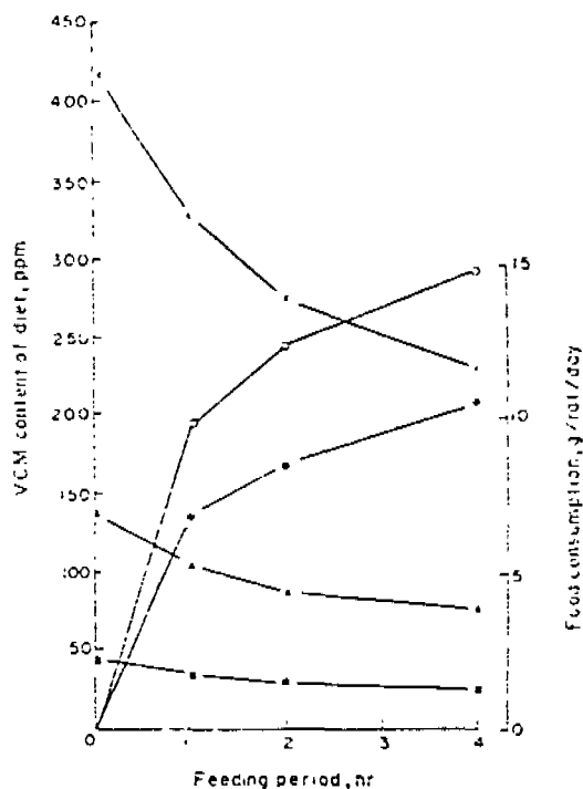
Fig. 1. Average VCM levels of the high-dose (▲), mid-dose (△) and low-dose (■) diets and average amounts of food consumed by males (○) and females (●) at different times during the 4-hr feeding period.
