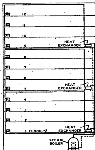
FIG. 17. VERTICAL ZONING OF HOT WATER HEATING SYSTEM IN A 12-STORY BUILDING connection. Short radiators are sometimes connected for top supply and bottom return on the same end. When so connected, attention must be given to venting of air from the top of the radiator somewhat oftener than when bottom connections are used.
