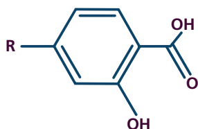
Figure 7. Typical Structure of a Salicylate Based Detergent
