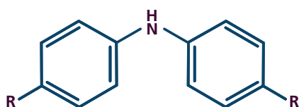
Figure 15. Diphenylamine
