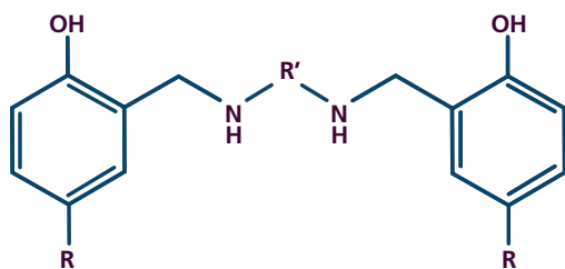
Figure 11. General Structure of a Mannich Base
