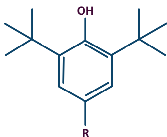
Figure 14. Hindered Phenol
