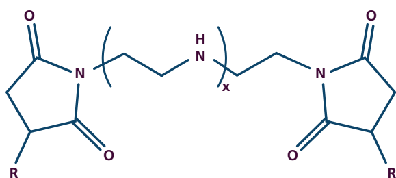
Figure 9. General Structure of a Succinimide Based Dispersant
