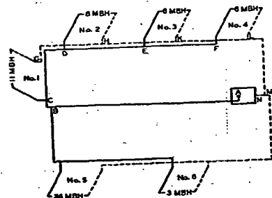
FIG. 13. TWO-PIPE REVERSED RETURN GRAVITY SYSTEM (EXAMPLE 5)
