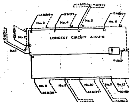
FIG. 14. FORCED CIRCULATION TWO-PIPE REVERSED RETURN SYSTEM
