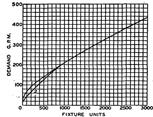
FIG. 1. ESTIMATE CURVES FOR DEMAND LOAD
